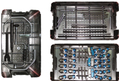
Large External Fixator Set H-Series
